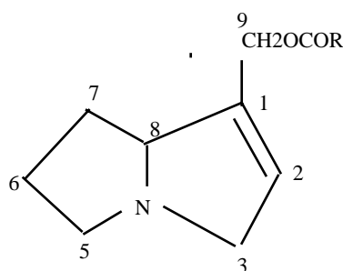
Figure 1. The basis structure of the hepatotoxic pyrrolizidine alkaloids
